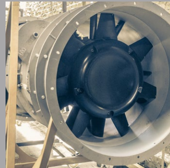
An MC1016 prior to mounting into the testing station.
